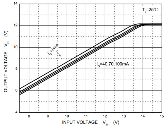
Figure 2. Dropout Characteristics
