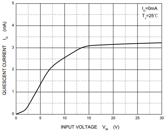
Figure 3. Quiescent Current
